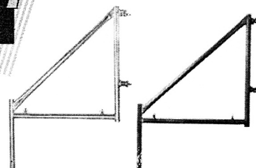
32" Outrigger Galvanized Finish M-M032GV
