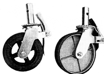
8" Caster, M-MBC8
