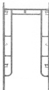
76" x 42" Walk-Thru Arch Frames M-MA7642GVPS
