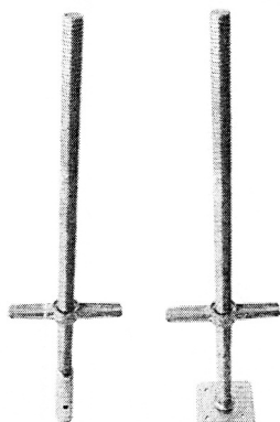
36" Galvanized Levelling Jack With Socket (Solid) M-MBSJS36
